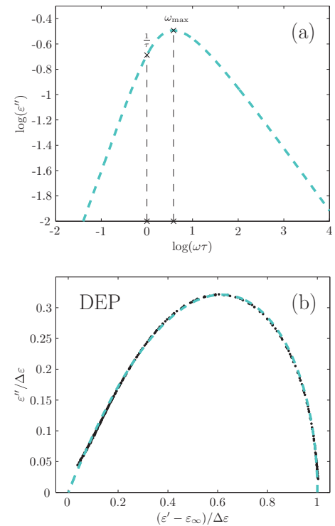
FIG. 10. (a) Illustration of the difference between the two calibrations of the dielectric relaxation rate \gamma_d , using either the loss-peak angular frequency or the rate of the long-time exponential decay of the dipole autocorrelation function giving the low-frequency Debye behavior. (b) Normalized Cole–Cole plot of the dielectric loss of DEP (black dots) vs that of the exponential \sqrt{t} relaxation function [Eq. (20)] used to fit the dielectric data at the following temperatures: 206, 207, 208, 209, 210, and 211 K (blue dashed line).
