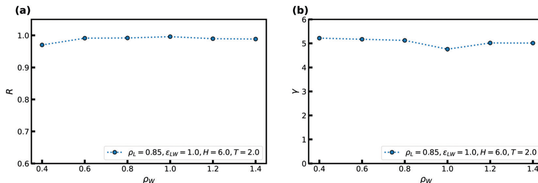
Fig. 4 The correlation coefficient R and density-scaling exponent \gamma as a function of crystal density \rho_W at T = 2 , H = 6 , and \varepsilon_{LW} = 1 . The liquid density is \rho_L = 0.85 . (a) R as a function of \rho_W . (b) \gamma as a function of \rho_W .
