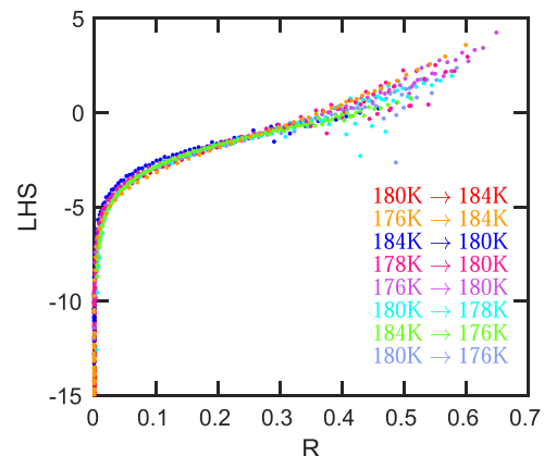
FIG. 5. Test 2. The left-hand side (LHS) of Eq. (10) plotted against R for all jumps. If the liquid obeys single-parameter aging, the data are predicted to collapse onto a master curve which is seen to apply to a good approximation.
