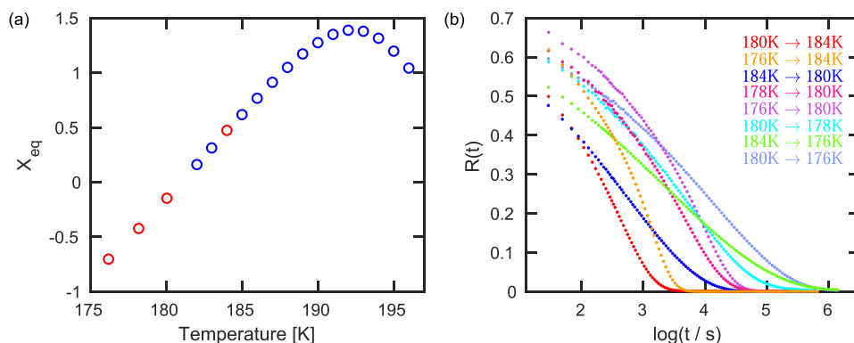
FIG. 2. Quantities used in the data analysis to perform the single-parameter tests. (a) The measured quantity [ \log(-\epsilon''(f = 0.1 \text{ Hz}, t)) ] at equilibrium at the final temperature ( X_{eq} ) as a function of temperature. The red circles indicate the four temperatures between which jumps are performed. The peak appearing between 190 K and 195 K is due to the \alpha -peak moving across the measuring frequency. (b) The normalized relaxation functions as functions of time for all jumps.
