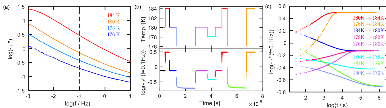
FIG. 1. Raw data. (a) The dielectric loss as a function of frequency at equilibrium at the temperatures the jumps are performed between. The dashed black line marks the frequency 0.1 Hz used for monitoring aging. (b) The temperature and the measured quantity [ \log(-\epsilon''(f = 0.1 \text{ Hz})) ] as functions of time. (c) The jumps on a logarithmic time scale. The data have been averaged in order to reduce noise as described in the text.
